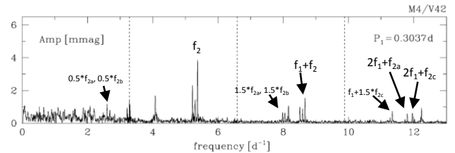
Fig. 4 Amplitude spectrum for RRc star V42. The first overtone radial mode and its harmonics have been removed, their locations are marked by the dotted lines. The thruster firing frequency at 4.08 c/d and its harmonics (8.16 c/d, 12.24 c/d) are very strong. A triplet of peaks is visible at f_{2a}=5.218 c/d, f_{2b}=5.298 c/d, and f_{2c}=5.373 c/d and corresponds to nonradial modes (see however Dziembowski 2016, Comm, Konkoly Obs. , 105, 23). The period ratios between these modes and the first radial overtone are 0.631, 0.622, and 0.613, and fall perfectly well on the three sequences in the Petersen diagram established by Netzel et al. 2015 ( MNRAS , 453, 2022). Nonradial modes with similar period ratios have been found in many RRc stars, but excitation of all three modes in a single star is rare. The three peaks at around 8.6 c/d are combination peaks of the first radial overtone and the triplet of nonradial modes. We also see subharmonics of the nonradial modes (two peaks at around 8.0 c/d and two peaks at around 2.6 c/d) and a combination peak involving one of the subharmonics (at 11.345 c/d).
