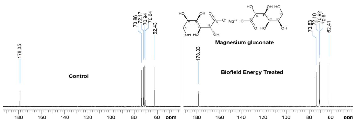
Figure 5. The 13 C NMR spectra of the control and Biofield Energy Treated magnesium gluconate.
