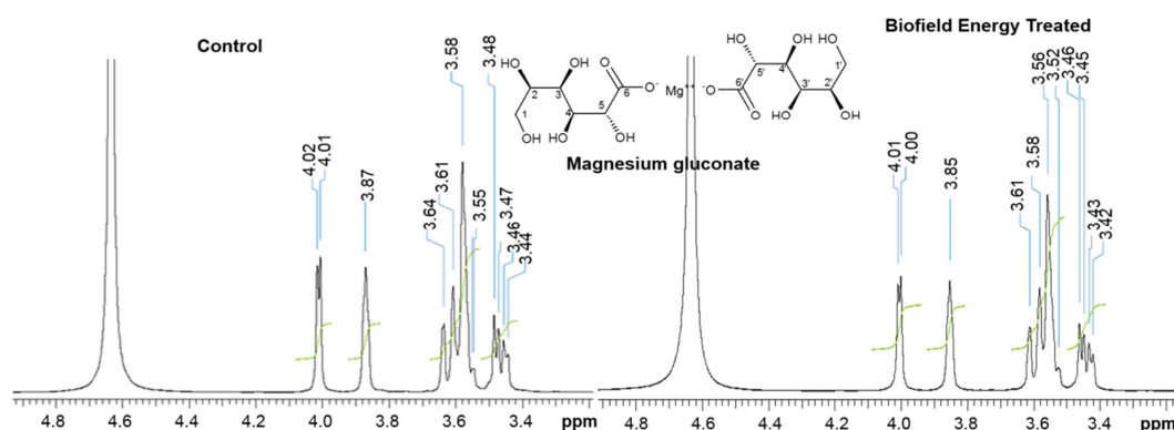
Figure 4. The 1 H NMR spectra of the control and Biofield Energy Treated magnesium gluconate.
