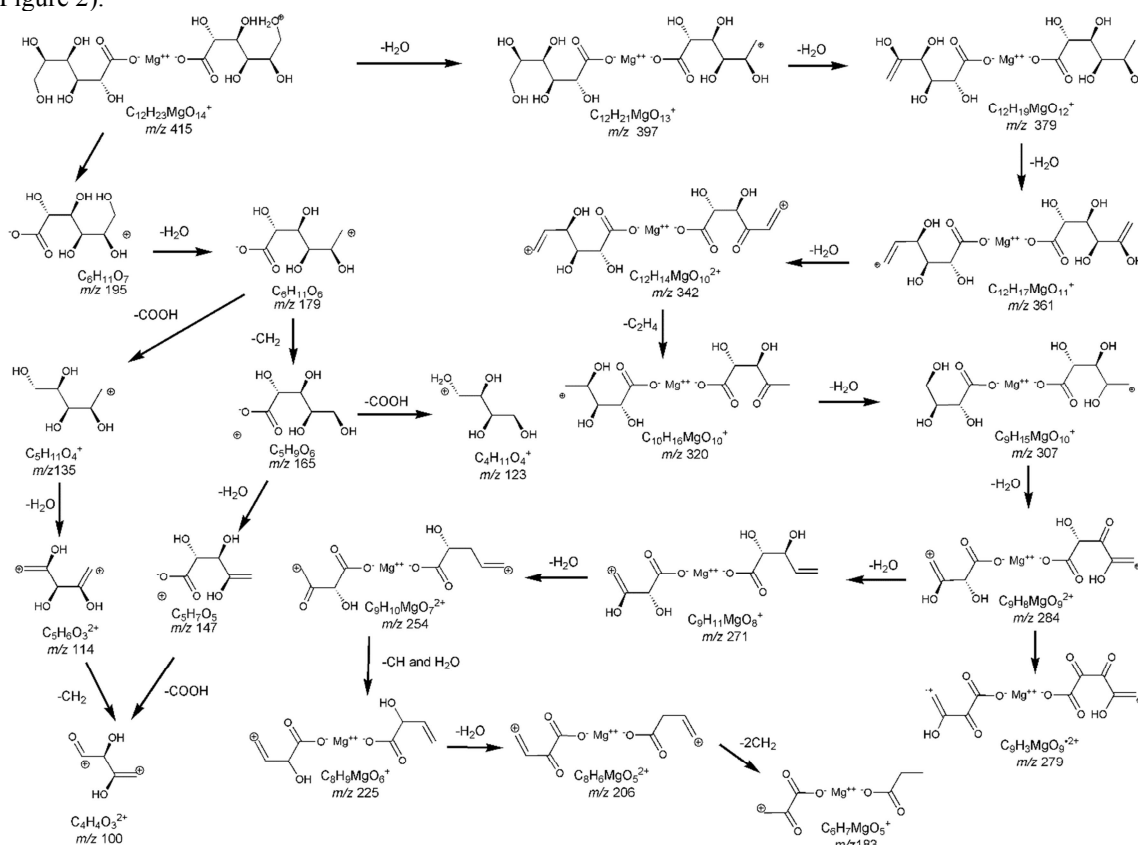
Figure 3. Proposed fragmentation pathway of magnesium gluconate.
