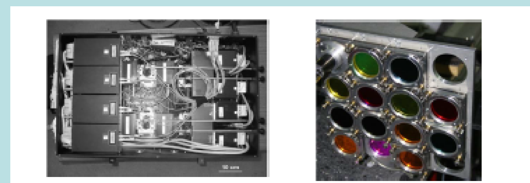
HELLRIDE Instrument Setup
