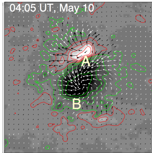
Photospheric Vector magnetgram
