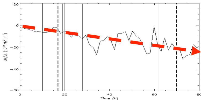
Injective mean magnetic helicity density
