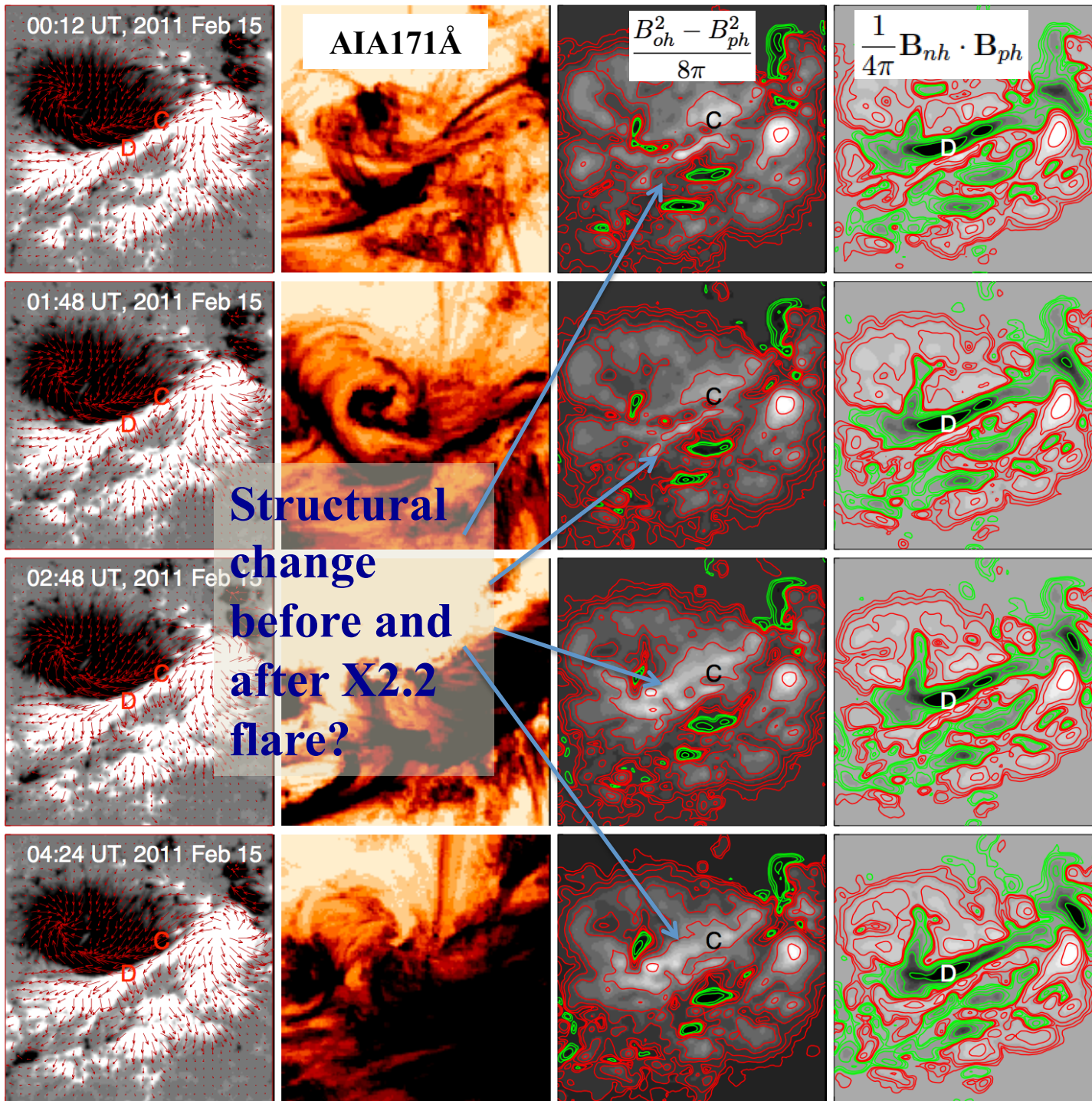
AR NOAA 11158 in 2011 February X2.2 flare (start at 01:44, peak at 01:45, end at 01:56 UT)
