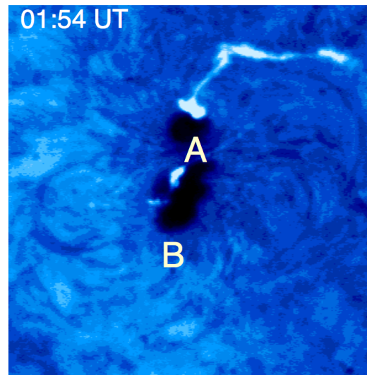
H \beta -chromospheric filtergram
