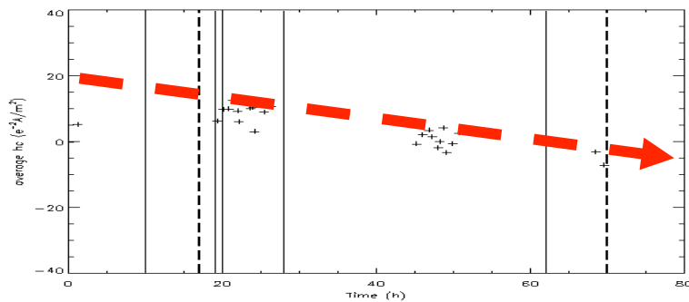
Evolution of mean current helicity density
