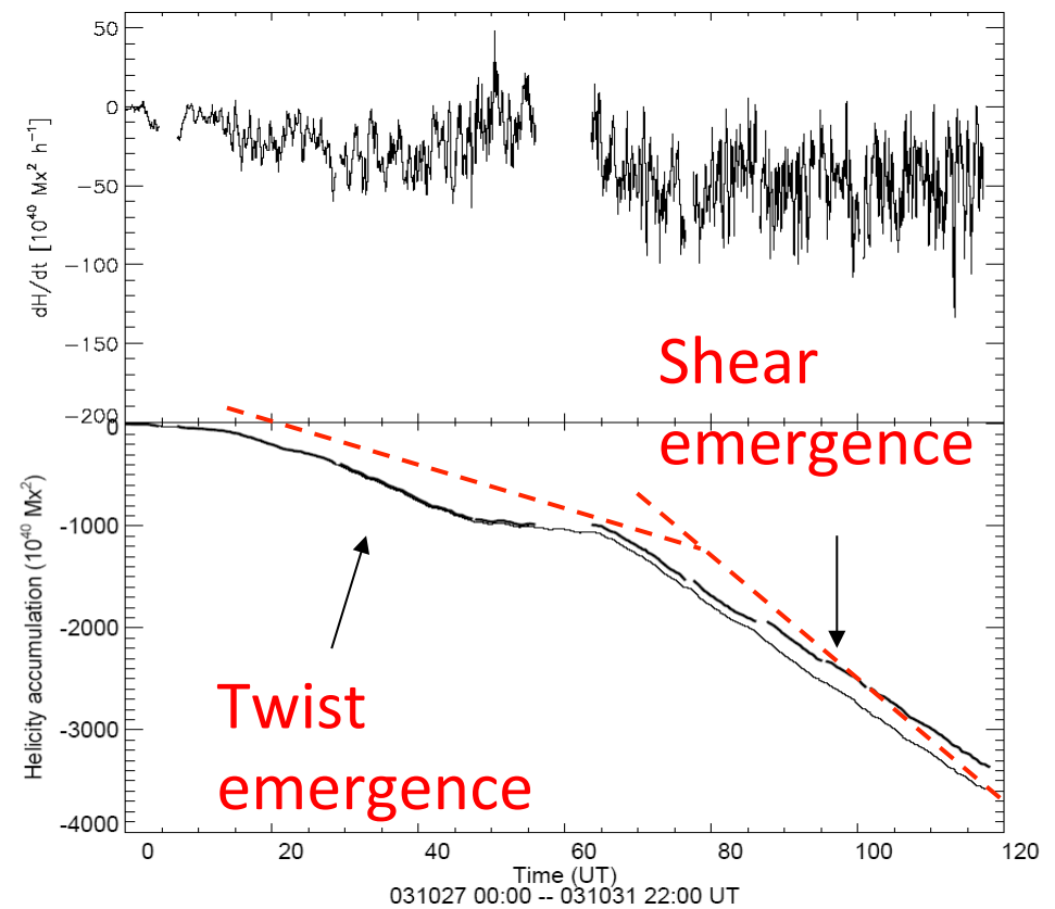
Accumulation of magnetic helicity from the subatmosphere
